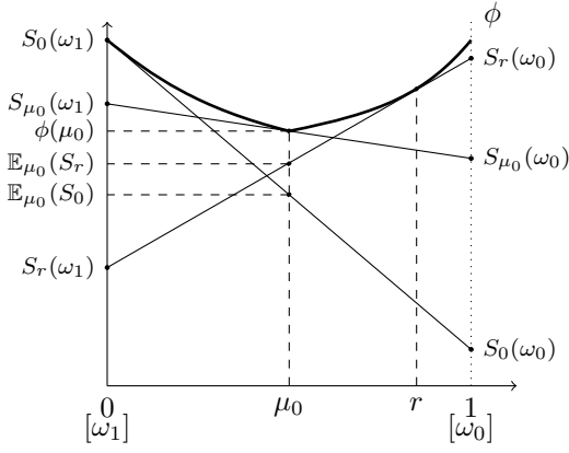
(a) PROPER SCORING RULE: The strictly convex function \phi(\mu) := \mathbb{E}_\mu(S_\mu) generates a proper scoring rule by taking an arbitrary tangent for each r and evaluating it at 0 and 1 respectively. Properness follows from the fact that the tangent at \mu_0 when evaluated at \mu_0 lies higher than the tangent at any other r when evaluated at \mu_0 , i.e., \mathbb{E}_{\mu_0}(S_{\mu_0}) > \mathbb{E}_{\mu_0}(S_r) .
