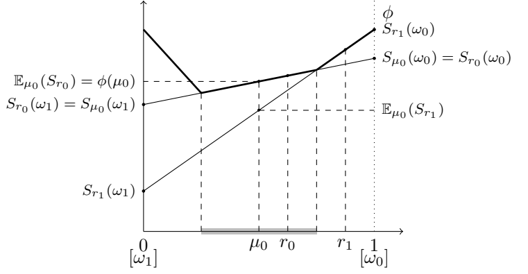
(b) WEAKLY PROPER SCORING RULE: The weakly convex function \phi(\mu) := \mathbb{E}_\mu(S_\mu) generates a weakly proper scoring rule by taking an arbitrary tangent for each r and evaluating it at 0 and 1 respectively. Weak properness follows from the fact that the tangent at \mu_0 when evaluated at \mu_0 lies at least as high as the tangent at any other r when evaluated at \mu_0 . The subject is indifferent among all reports in the shaded subinterval I_\phi(\mu_0) , i.e., \mathbb{E}_{\mu_0}(S_{\mu_0}) > \mathbb{E}_{\mu_0}(S_{r_1}) while \mathbb{E}_{\mu_0}(S_{\mu_0}) = \mathbb{E}_{\mu_0}(S_{r_0}) .
